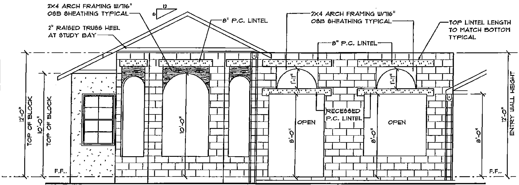
ENTRY FRAMING
