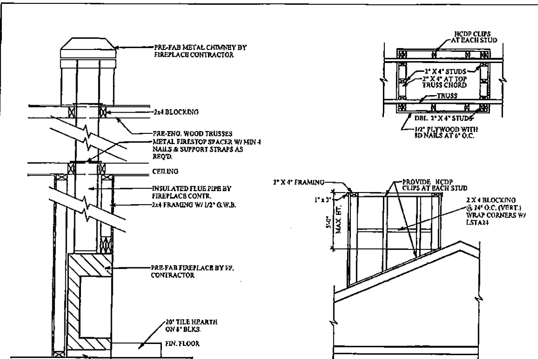
SECTION - FIREPLACE
