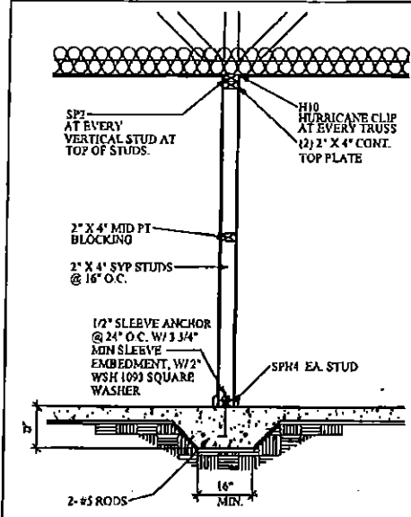
BEARING PARTITION
