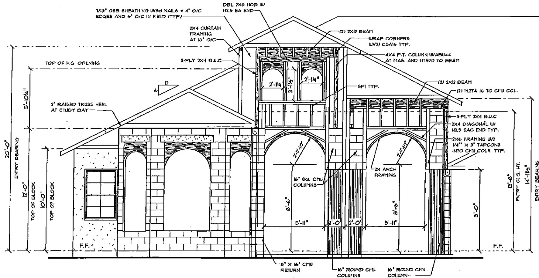
ENTRY FRAMING
