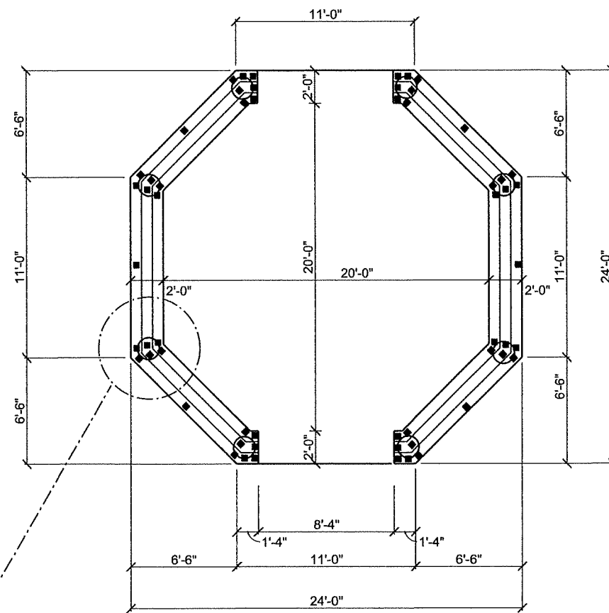
FLOOR PLAN
