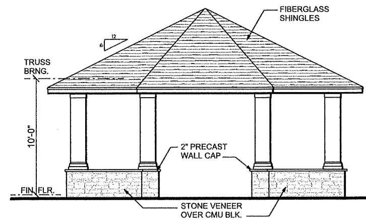
EXTERIOR ELEVATION
