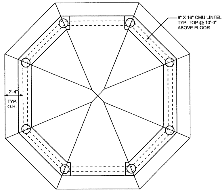
ROOF PLAN
