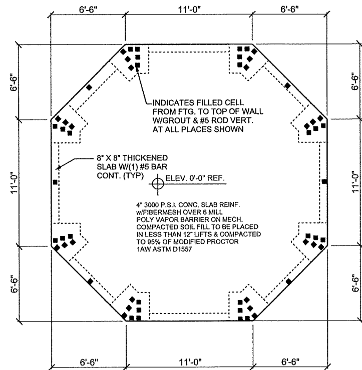
FOUNDATION PLAN
