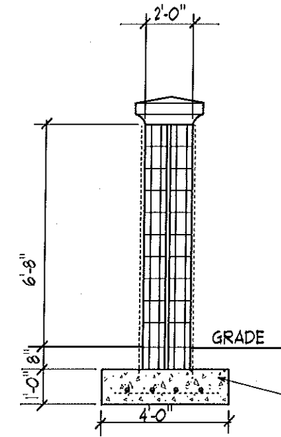
TYPICAL COLUMN
